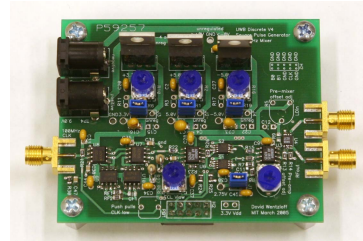
Fig. 5. Pulse generator.
