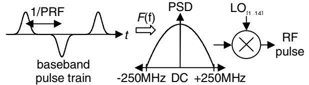
Fig. 1. Baseband Gaussian pulse train with BPSK modulation.
